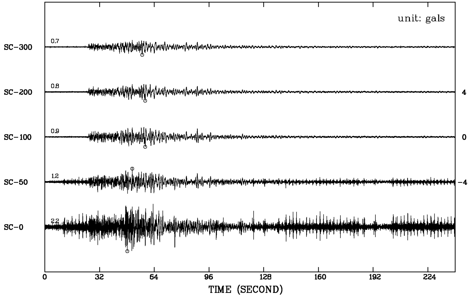
The particle accelerations recorded by the TBDA on EQ201303270203 V
