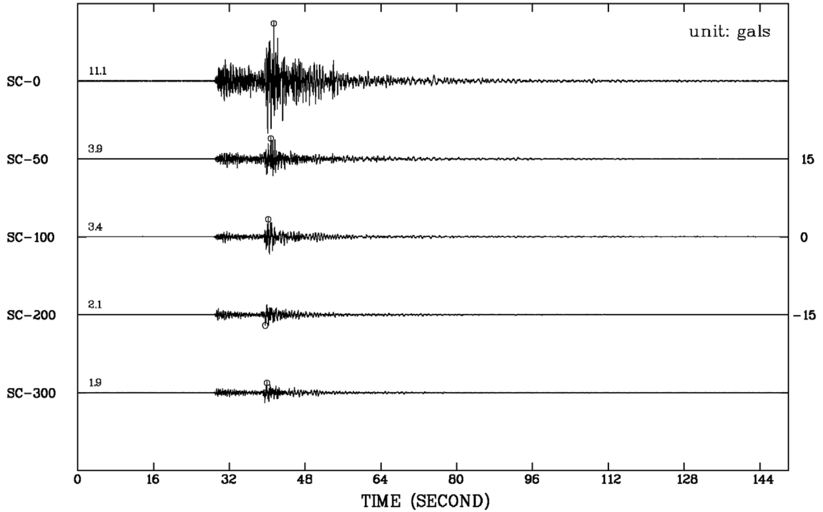
The particle accelerations recorded by the TBDA on EQ200806011659 EW
