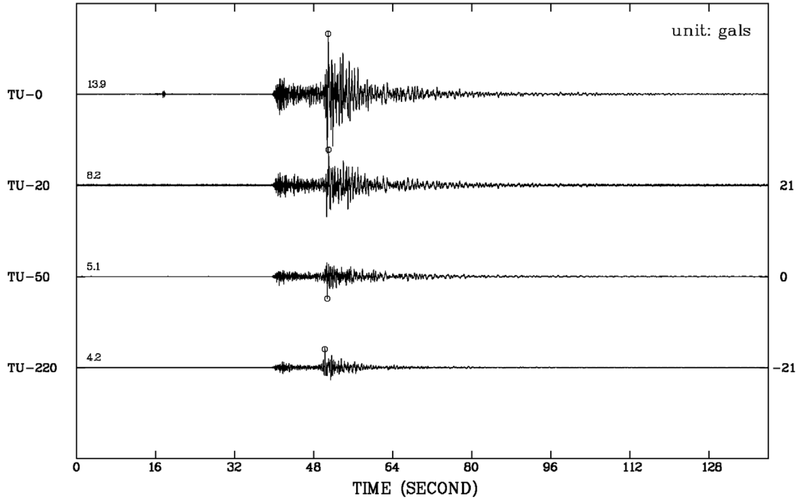
The particle accelerations recorded by the TBDA on EQ200806011658 EW
