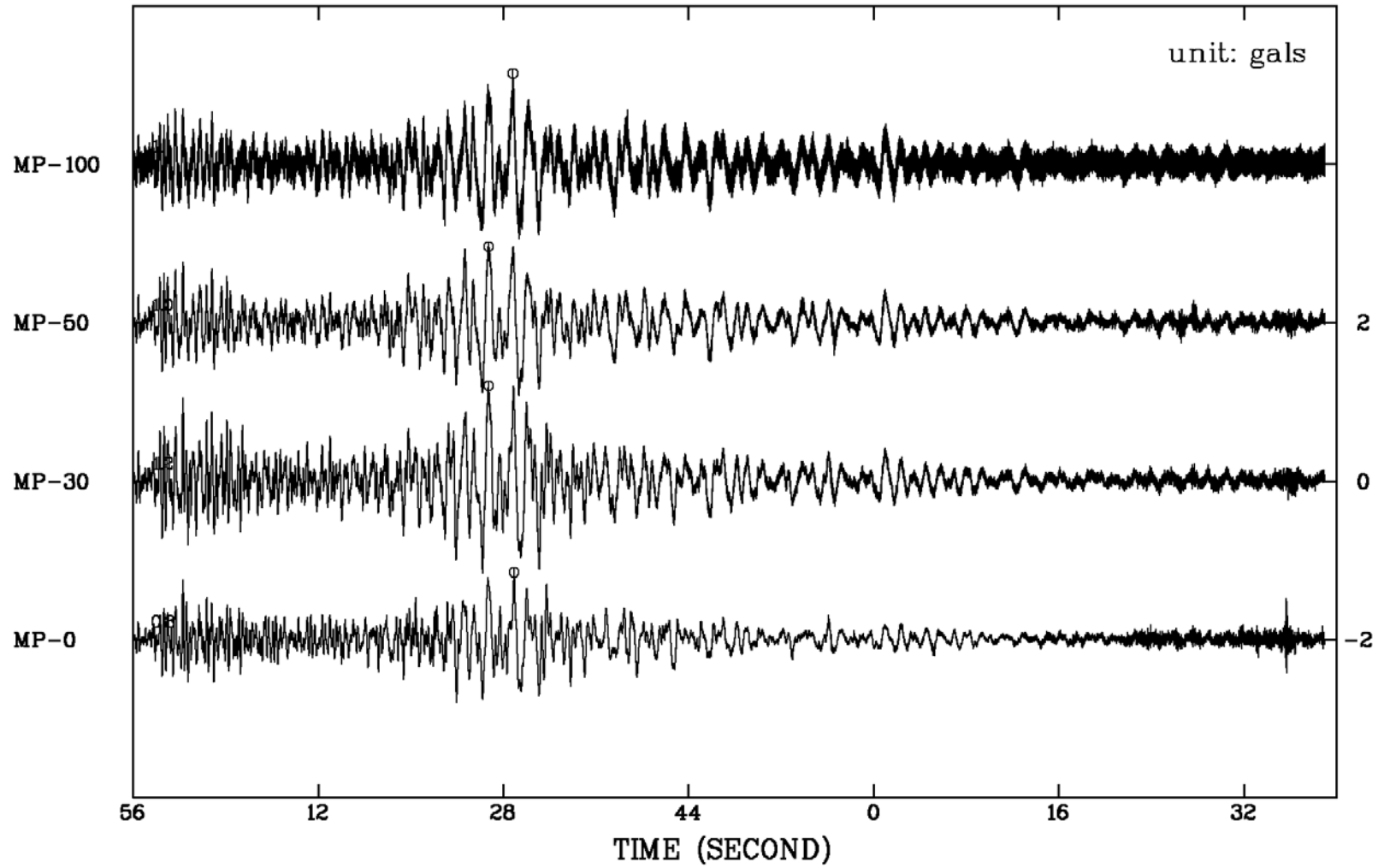
The particle accelerations recorded by the TBDA on EQ200610121446 V
