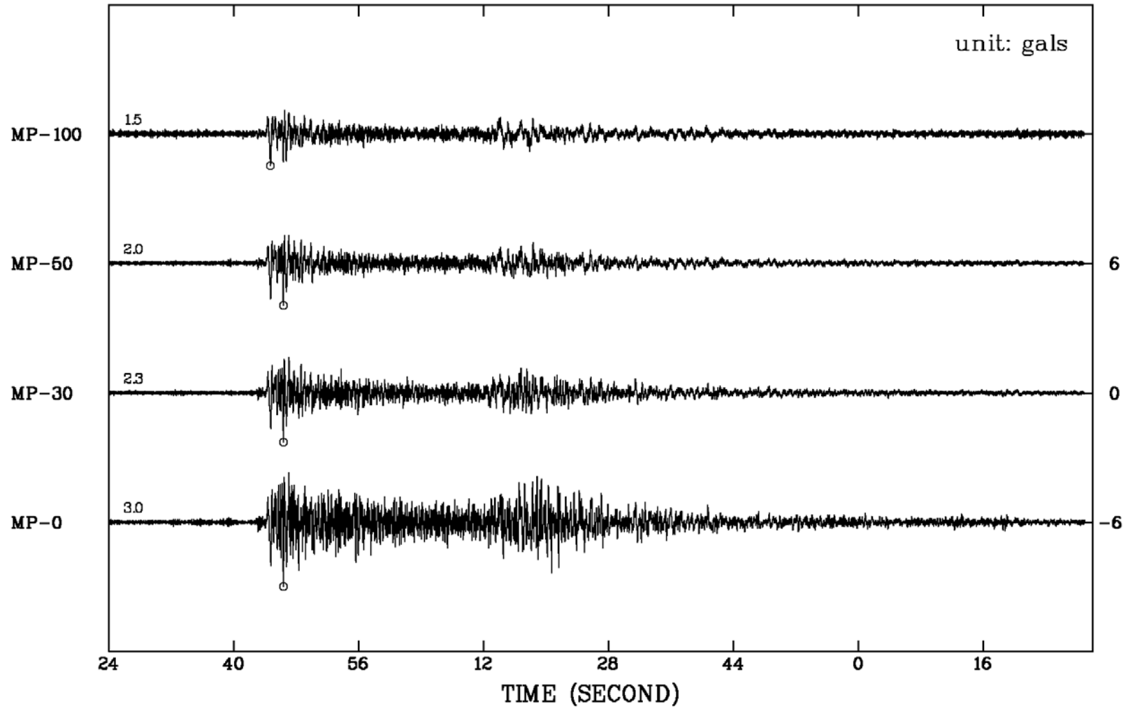
The particle accelerations recorded by the TBDA on EQ200510151551 V
