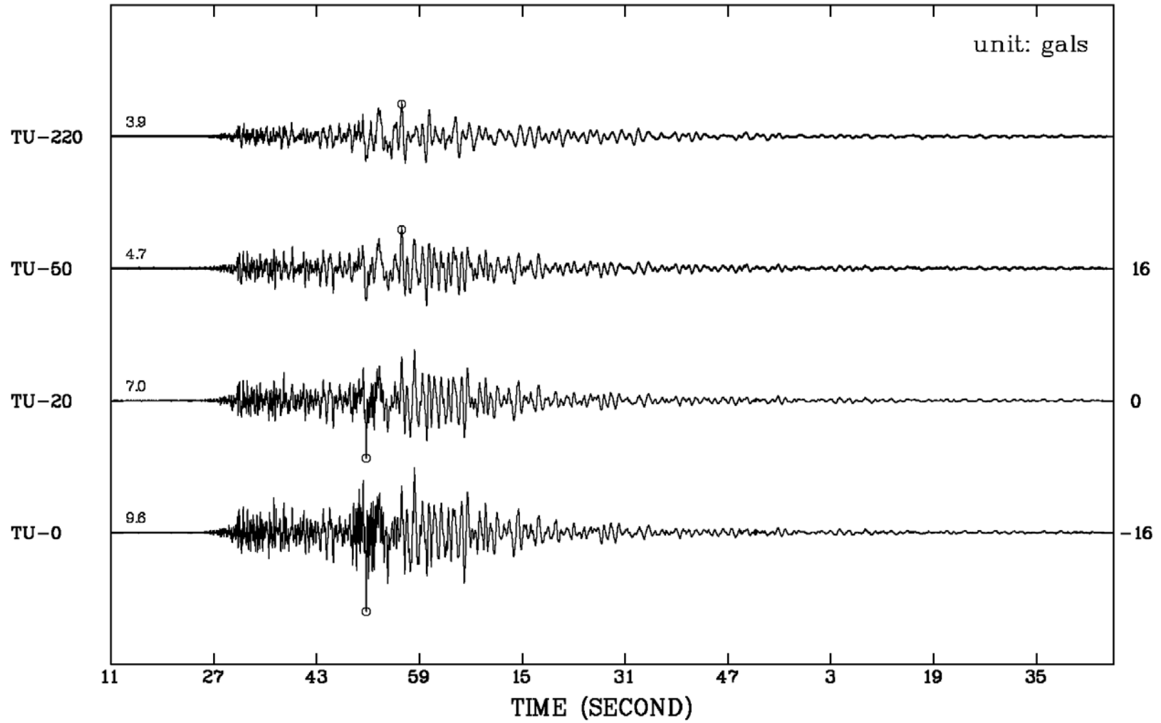
The particle accelerations recorded by the TBDA on EQ200411081555 V
