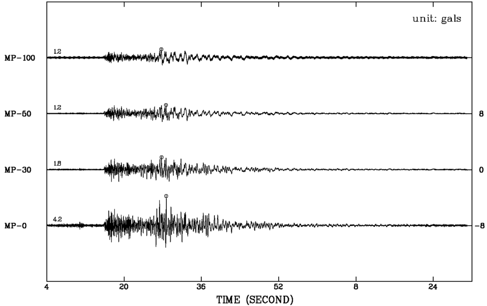
The particle accelerations recorded by the TBDA on EQ200407060732 V
