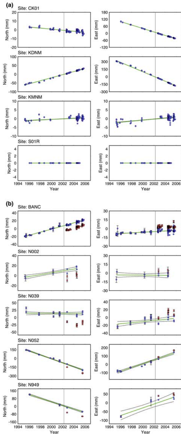
Figure 3. Coordinate time series of the selected GPS stations. Red circles are original observations. Blue circles indicate the corrected data in which the coseismic offsets of 2002 Hualien, Taiwan offshore earthquake were removed. The gray lines represent the occurrence epoch of the 2002 Hualien, Taiwan offshore earthquake. Green lines are the best-fitting lines using the least squares method. Black dashed lines denote a 95% confidence interval. (a) Coordinate time series of the constrained local permanent GPS stations. (b) Coordinate time series of the selected campaign-surveyed GPS stations. The coordinate time series of the station BANC denotes the best case while the time series of the site N949 shows the worst case.
